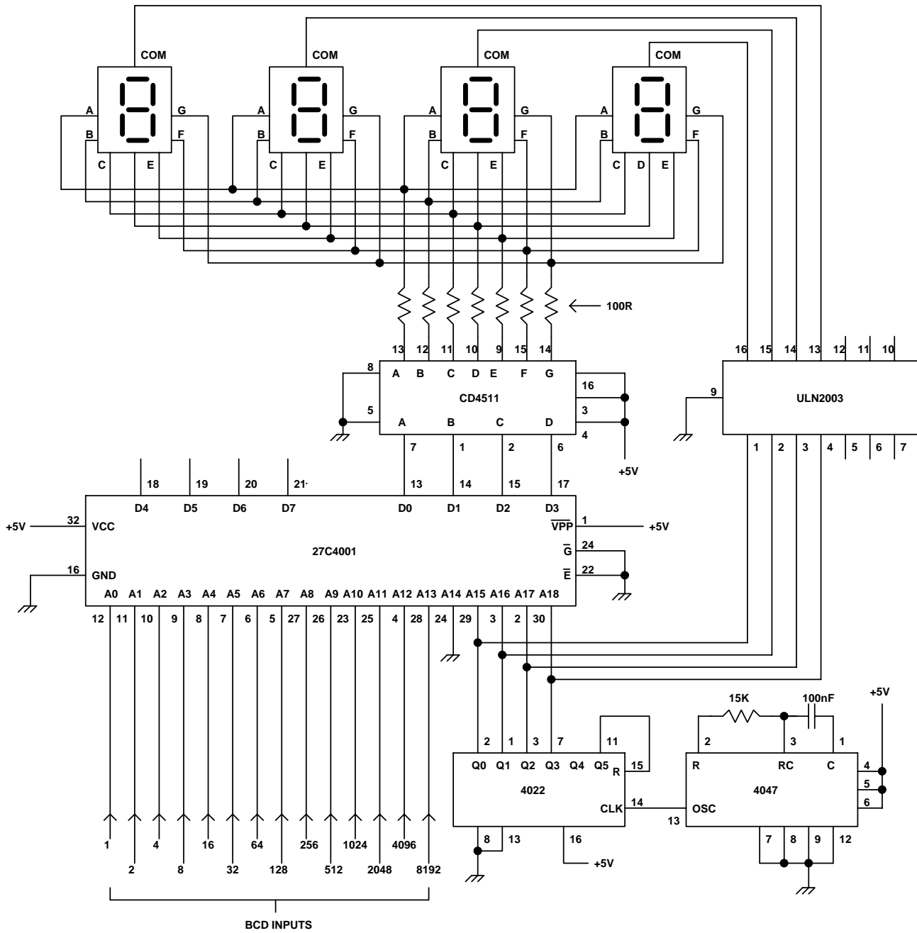
7 BIT BCD TO DECIMAL DECODER USING AN EPROM (0000 TO 9999)
